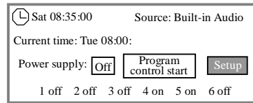
Fig. 1: Main interface
