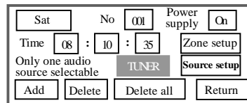
Fig. 5: Timer setting interface
